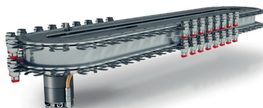
Chain magazine and tool changer
