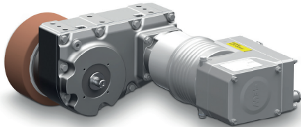
Optional second shaft end e.g. for encoder mounting
